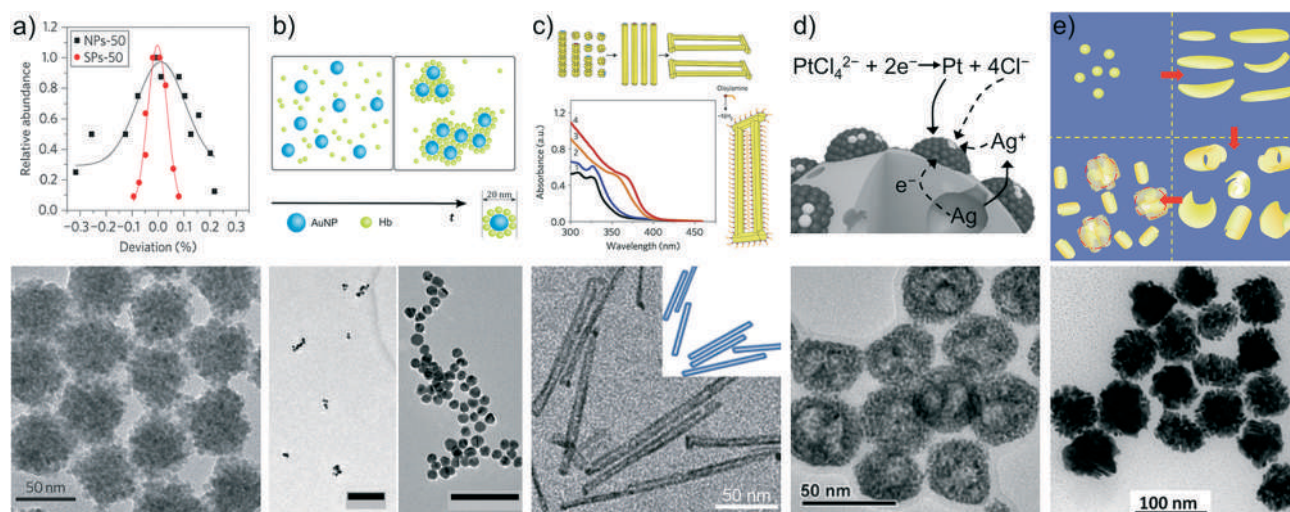
Fig. 1 a) Self-assembly of CdTe nanoparticles into spherical and uniform supraparticles exhibiting a significant reduction in polydispersity. b) Agglomeration of gold nanoparticles at high (left) and low (right) hemoglobin concentrations. c) Growth stages of the high-temperature assembly of ZnSe nanoparticles (top) leading to couples of colloidal nanorods (bottom). d) Mesoporous surfactant-free colloids made of platinum-group nanocrystals obtained through coprecipitation on silver particles as sacrificial substrates. e) Growth mechanism of “meatball”-like gold supraparticles synthesized by a seed-mediated approach. Figures reproduced with permission from ref. 11, 19, 23, 28 and 18. Copyright 2012 and 2014 Nature Publishing Group; Copyright 2015 American Chemical Society; Copyright 2015 Wiley-VCH Verlag GmbH & Co. KGaA.
