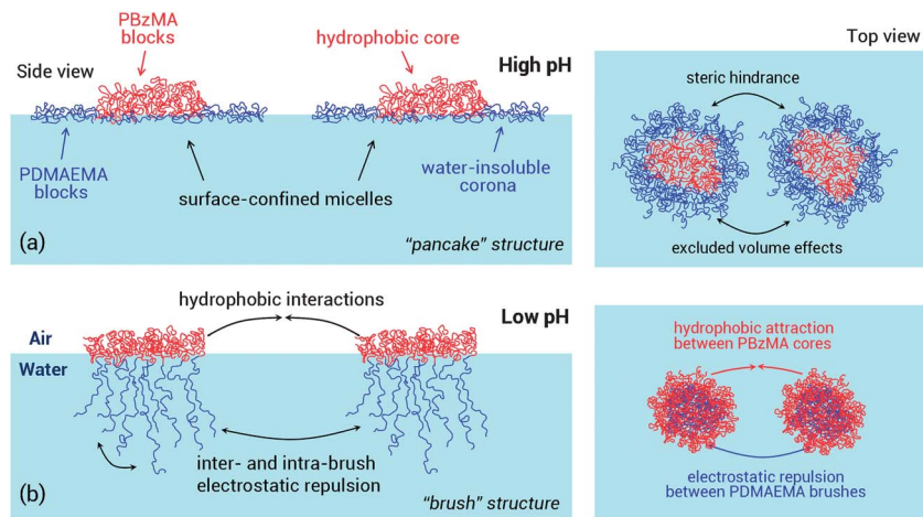
Fig. 2 Schematic illustrations (side and top views) of surface micelles formed at the air–water interface under (a) high and (b) low pH conditions.
